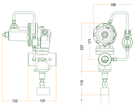
629 Shutoff 1"
